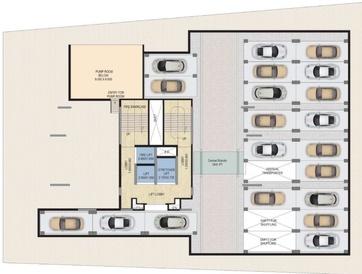
BASEMENT PLAN
